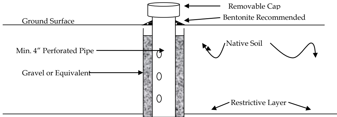
FIGURE 1 EXAMPLE SOIL/GROUNDWATER OBSERVATION WELL CONSTRUCTION
